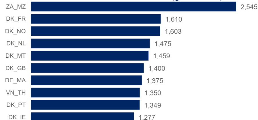
Emission factor - Ø CO2e WTW (g/tonne-km)
