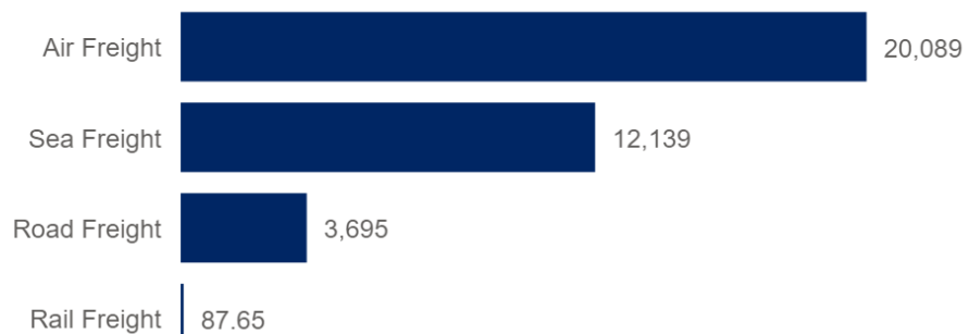
SO2 WTW (kg)
