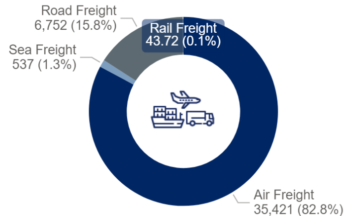
CO2e WTW (t) by Transport Mode
